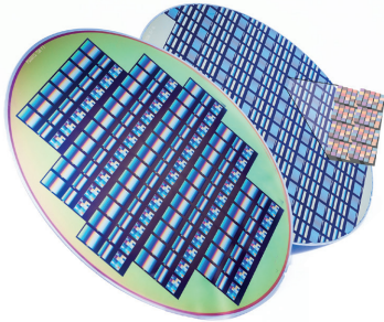
imec hyperspectral imager structures processed at wafer-level on top of commercial CMOS image sensor wafer
